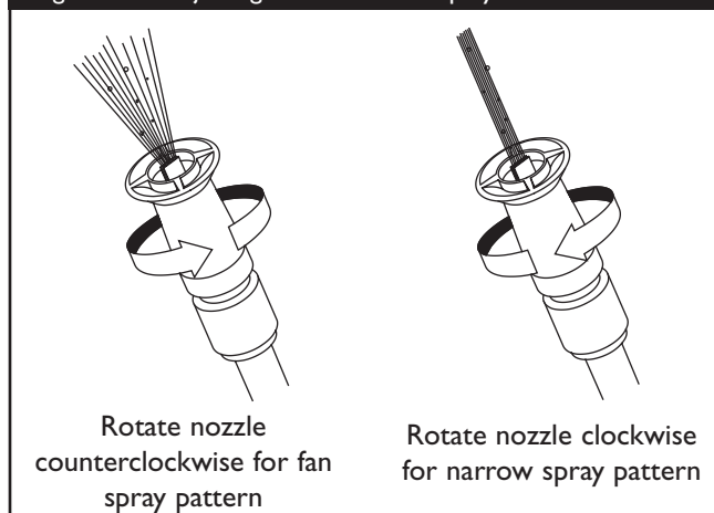
Figure 8 — Adjusting the Nozzle for Spray Pattern
