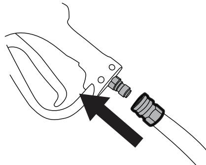
Figure 11 – Connect Hose to Spray Gun
