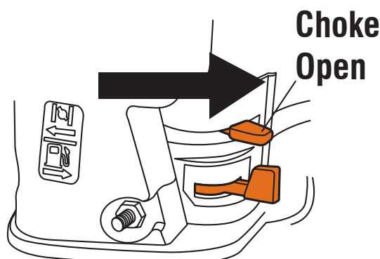
Figure 25 – Choke Lever
