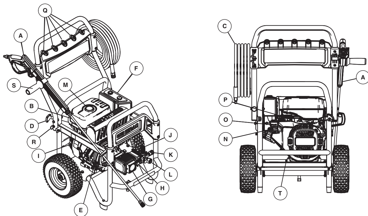
Figure 1 – Features & Controls
