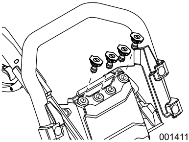
Figure 2-3. Insert Nozzles
