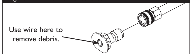
Figure 10 — Nozzle Maintenance
