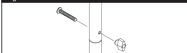
Figure 2 — Secure Handle
