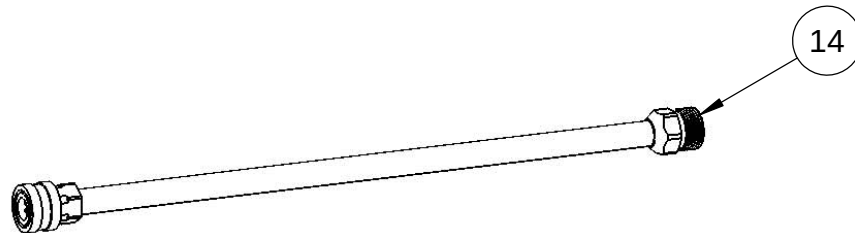
LANCE, 16" W/ 1/4"QC-F x M22(M) PART NO. 7103550
