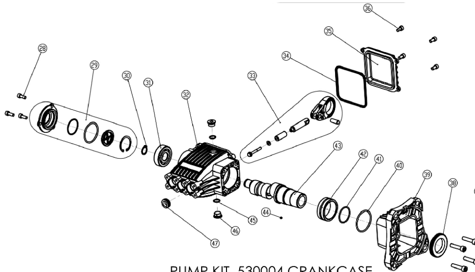
PUMP KIT, 530004 CRANKCASE PART NO. 7107347 #530004 PUMP DRAWING PARTS
