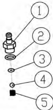
25 PART NO. 7104228
