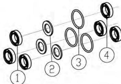
14 PART NO. 7106627
