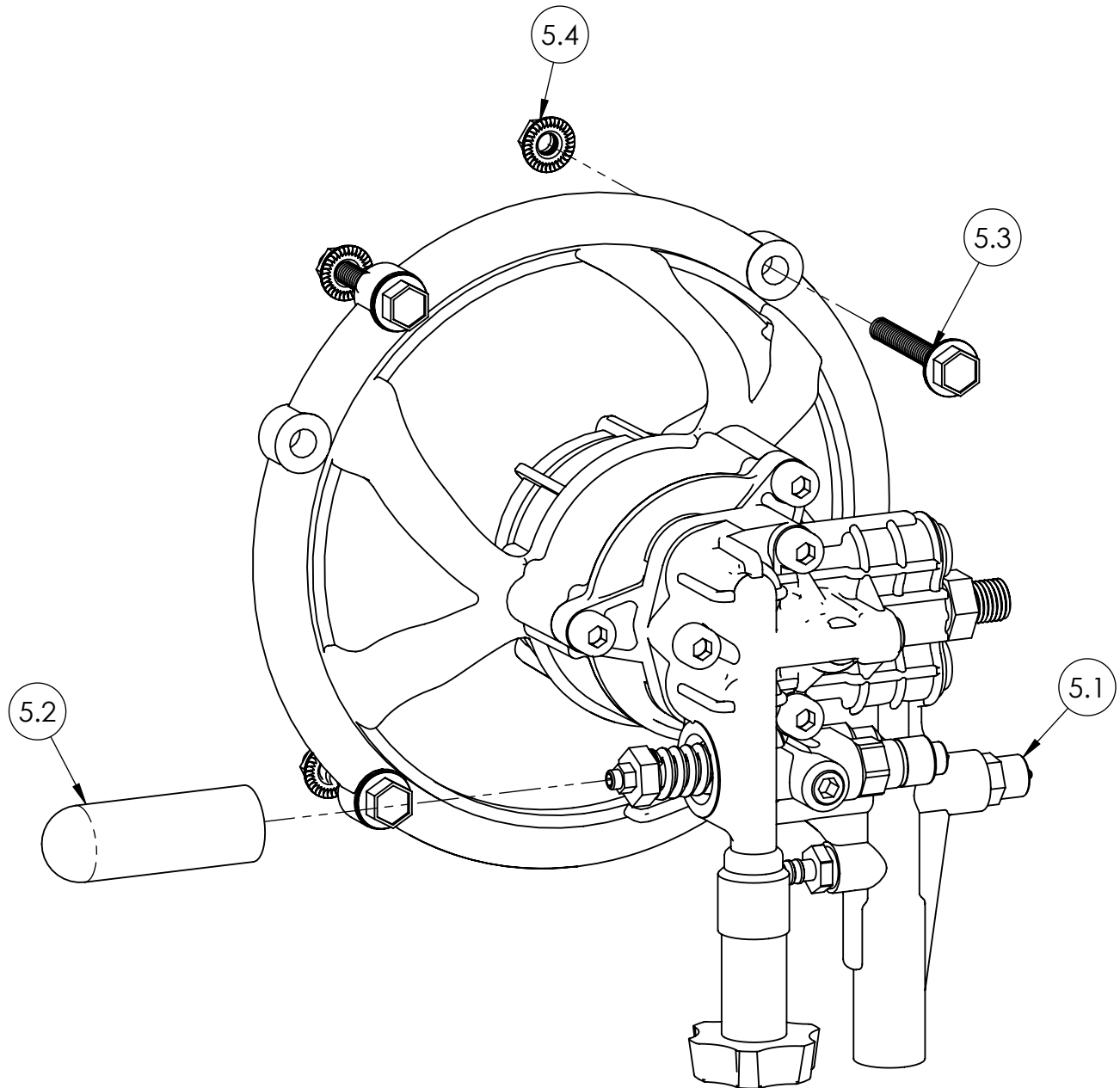
PUMP, SVC ASSY MSV3024-I PART NO. 7107839
