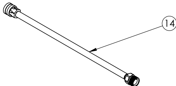
LANCE, 16" W/ 1/4" QC-F X M22(M) PART NO. 7103550
