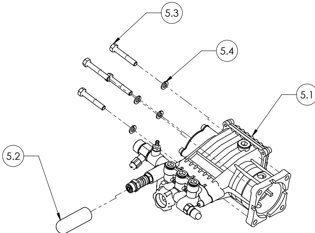
PUMP, SERVICE ASSY KIT PART NO. 7106596
