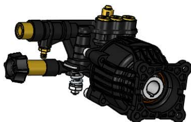
⑥.1 PUMP, HORZ, 12mmx12DEG, P/B, AL UNIHEAD PART NO. 520004
