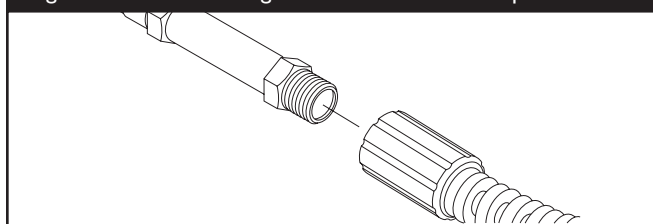
Figure 5 — Connect High Pressure Hose to Pump
