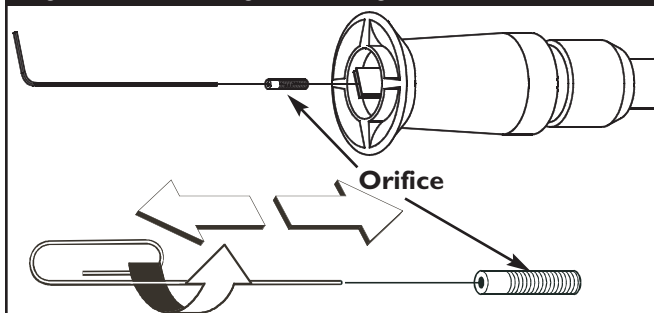
Figure 13 — Removing and Cleaning Orifice
