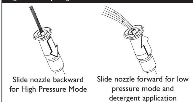
Figure 9 — Adjusting Nozzle for Pressure
