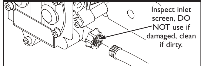
Figure 10 — Connect Garden Hose to Water Inlet
