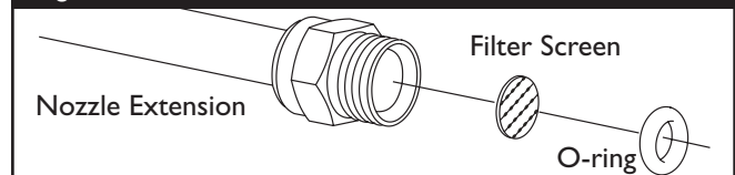
Figure 17 — Clean In-Line Filter
