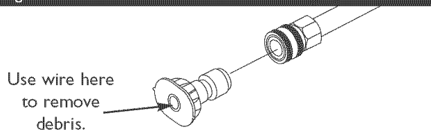
Figure 21 — Nozzle Maintenance
