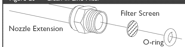
Figure 20 — Clean In-Line Filter
