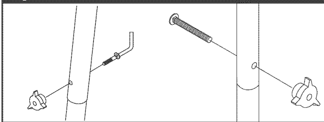
Figure 3 — Secure Handle
