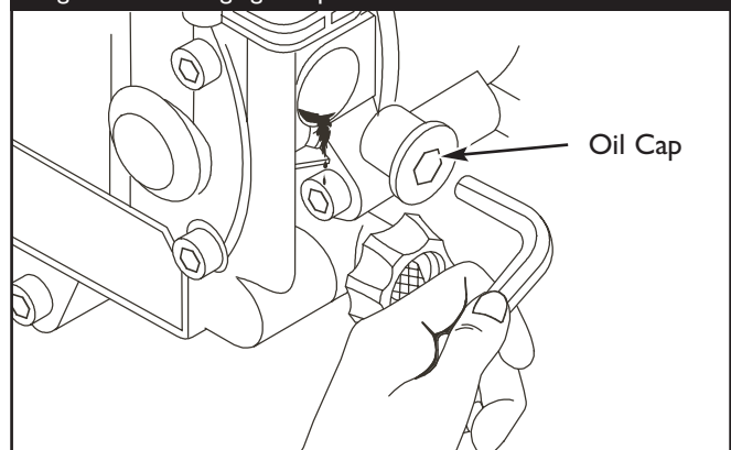
Figure 20 - Changing Pump Oil
